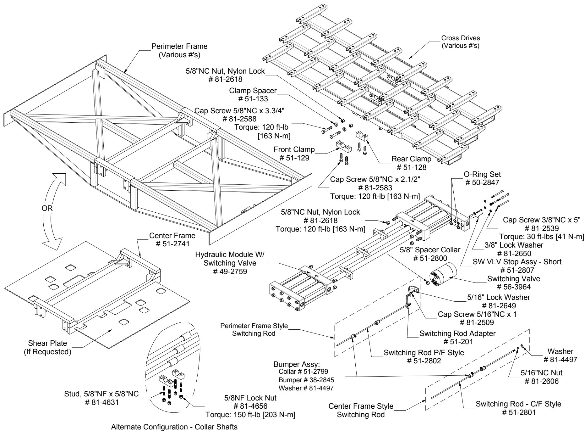
-Figure 4- Drive Unit--Exploded View
