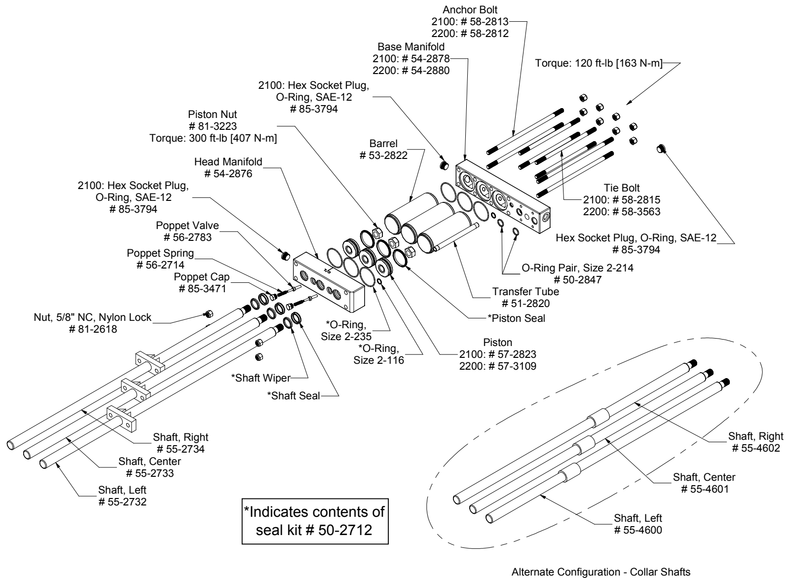
-Figure 10- 2000 Series Hydraulic Module--Exploded View
