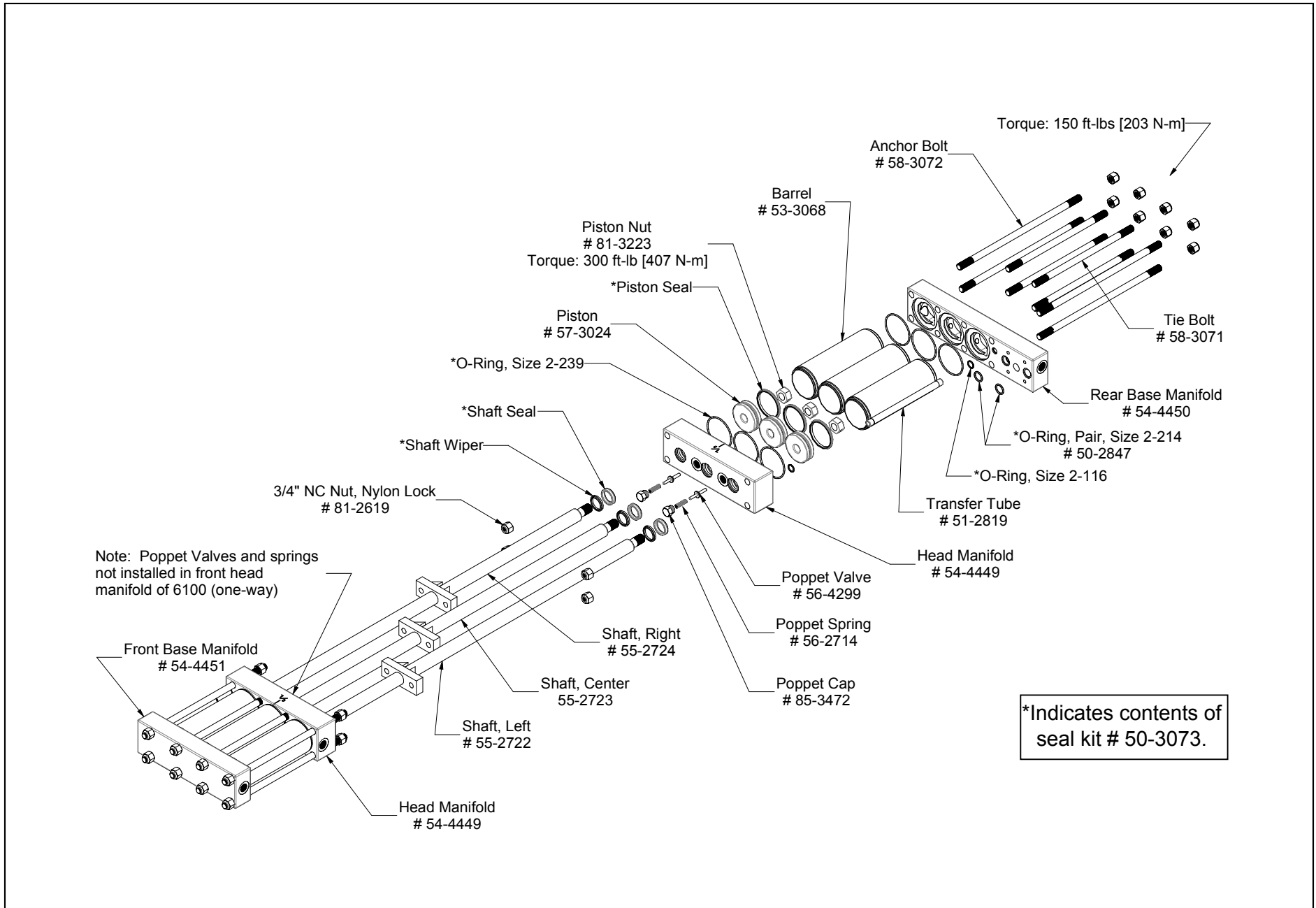
-Figure 10- 6000 Series Hydraulic Module--Exploded View
