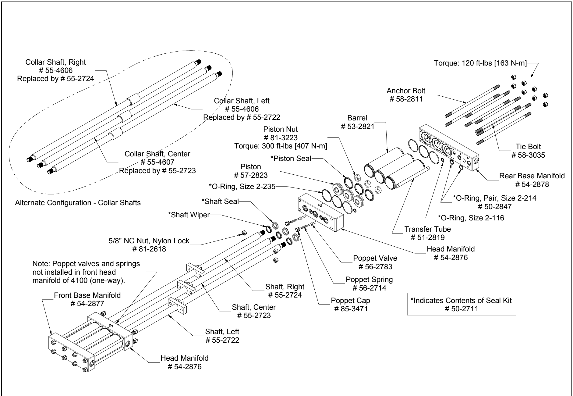
-Figure 10- 4000 Series Hydraulic Module--Exploded View
