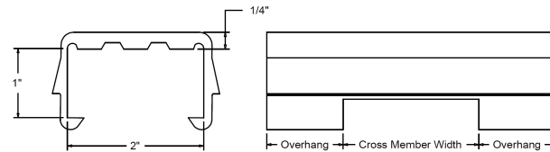
Continuous Bearing (9 Ft Lengths) P/N 39-4093
