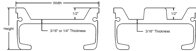
"X" Seal P/N 39-4007
